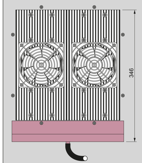
TCU200 / TCU200AC max. height with drip tray
