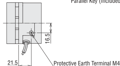
Detail Drawing of Protective Earth Terminal
